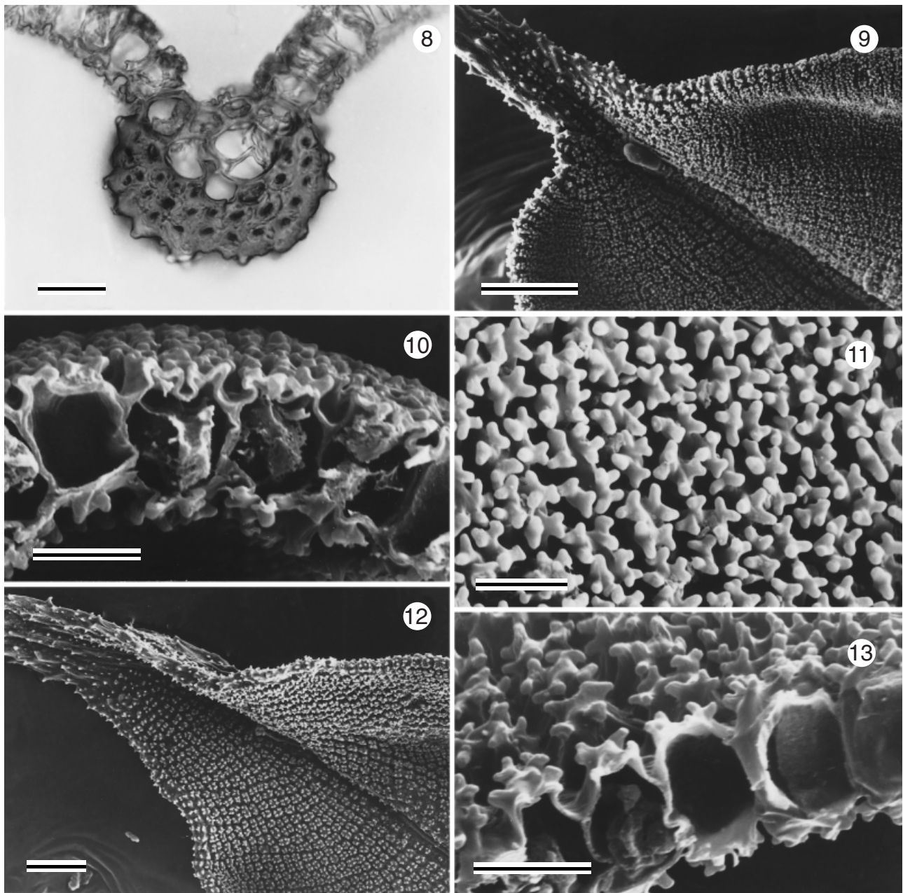
Figures 8–13. Syntrichia ruralis MUB 2717. Fig. 8. Transverse section (TS) of the leaf. Scale bar = 30 \mu m. Fig. 9. Leaf apex. Scale bar = 100 \mu m. Fig. 10. TS lamina cells. Scale bar = 10 \mu m. Syntrichia ruralis var. ruraliformis MUB 1139. Fig. 11. Lamina cells. Scale bar = 10 \mu m. Fig. 12. Leaf apex. Scale bar = 50 \mu m. Fig. 13. TS lamina cells. Scale bar = 10 \mu m.
