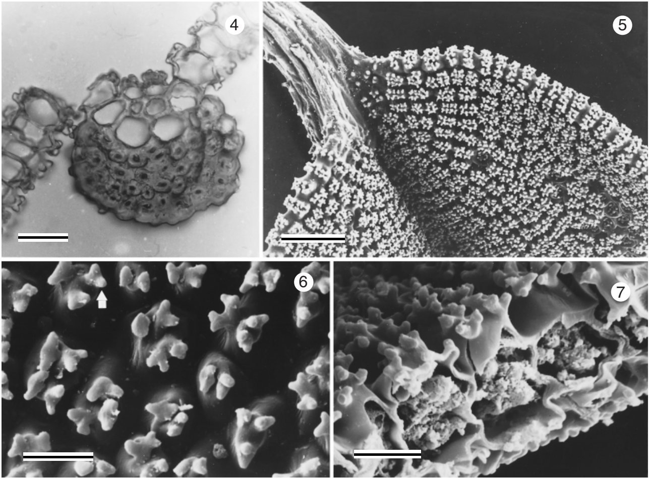
Figures 4–7. Syntrichia calcicola MUB 10382. Fig. 4. Transverse section (TS) of the leaf. Scale bar = 30 µm. Fig. 5. Leaf apex. Scale bar = 50 µm. Fig. 6. Lamina cells. Scale bar = 10 µm. Fig. 7. TS of the lamina cells. Scale bar = 10 µm.
